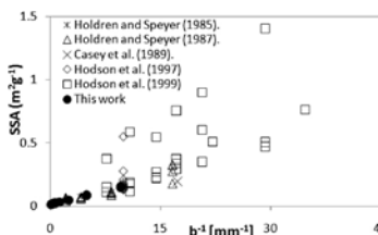
Figure 4. Specific surface area of sanidine as a function of the inverse of the particle size. Data from this study and the literature.
